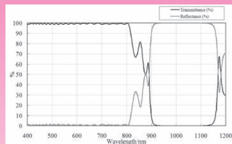
YAG Laser Mirror
