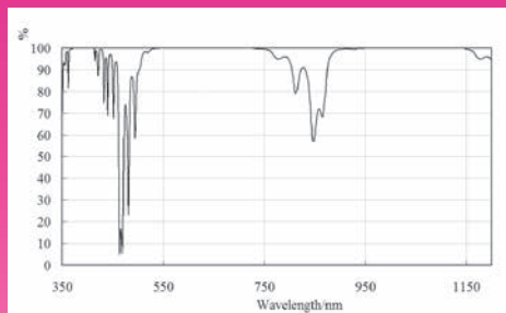
3 Wavelength Laser Mirror
